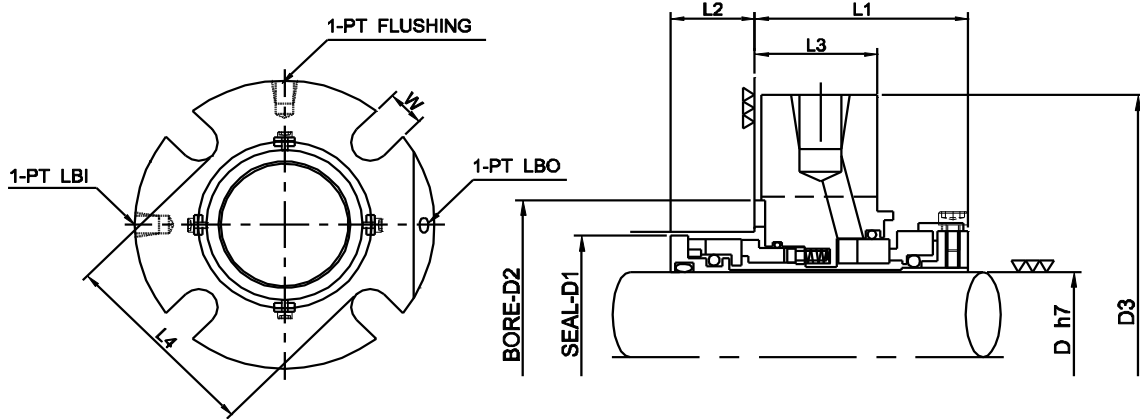
Type FW520 dimensions
